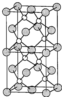
Spalrite, B3 ZnS
