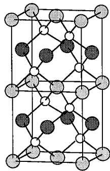
layered tetragonal, L1 0 InGaAs 2
