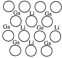
\beta -LiGaO 2
